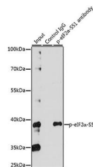
Fig. 2. Immunoprecipitation analysis of 200 \mu g extracts of HeLa cells, using 3 \mu g Phospho-eIF2 \alpha -S51 pAb at a dilution of 1:1000. HeLa cells were treated by Calyculin A at 37°C for 30 minutes after serum-starvation overnight.
