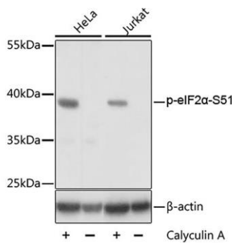
Fig. 1. Western blot analysis of extracts of HeLa and Jurkat cells, using Phospho-eIF2 \alpha -S51 antibody at 1:2000 dilution. HeLa cells were treated by Calyculin A for 30 minutes after serum-starvation overnight. Jurkat cells were treated by Calyculin A for 30 minutes. Secondary antibody: HRP-labeled Goat Anti-Rabbit IgG(H+L) (A0208) at 1:1000 dilution. Lysates/proteins: 25 \mu g per lane. Blocking buffer: QuickBlock™ Blocking Buffer (P0231). Detection: BeyoECL Star (P0018A). Exposure time:1s.
